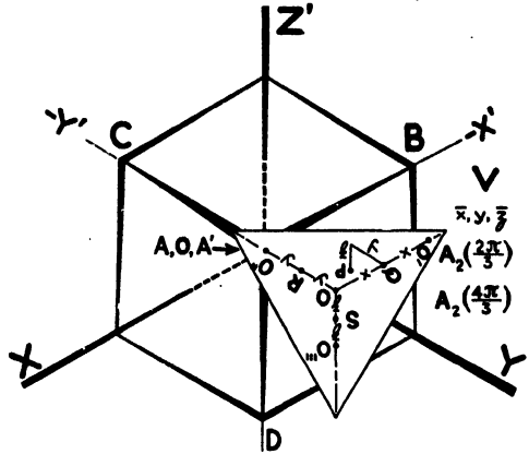
FIG. 8.—The template after Umlappung about the Y-axis.
